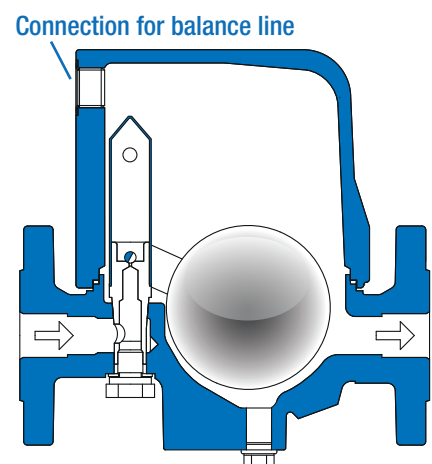
Model WU as feed control
